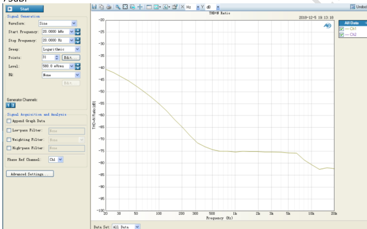
Fig. 4-22 Audio recording path THD+N ratio at differential mode
